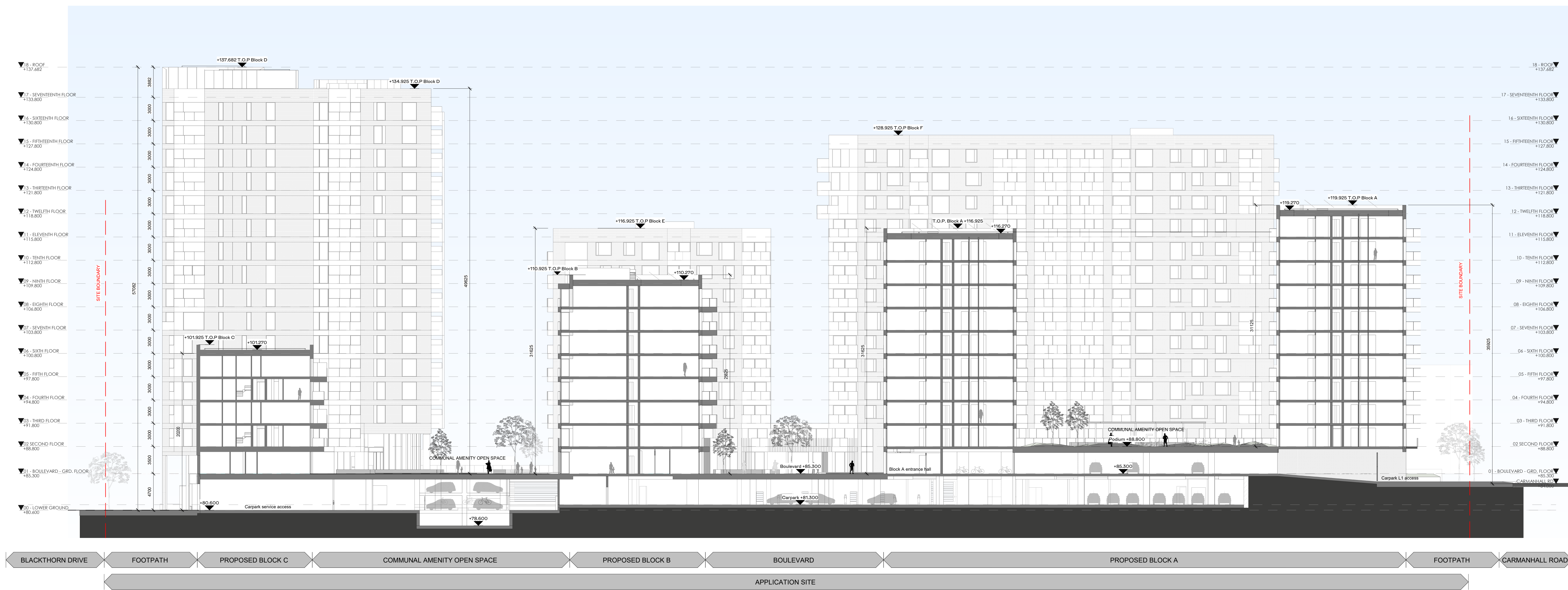
04 Section 04 1:500
